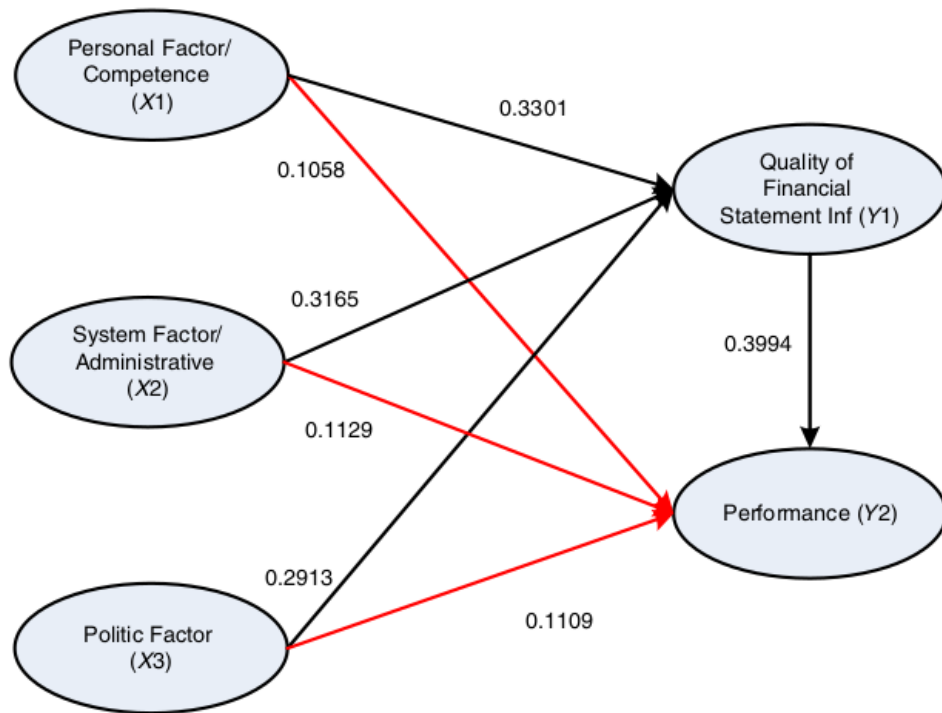
Figure 2. PLS structural model
